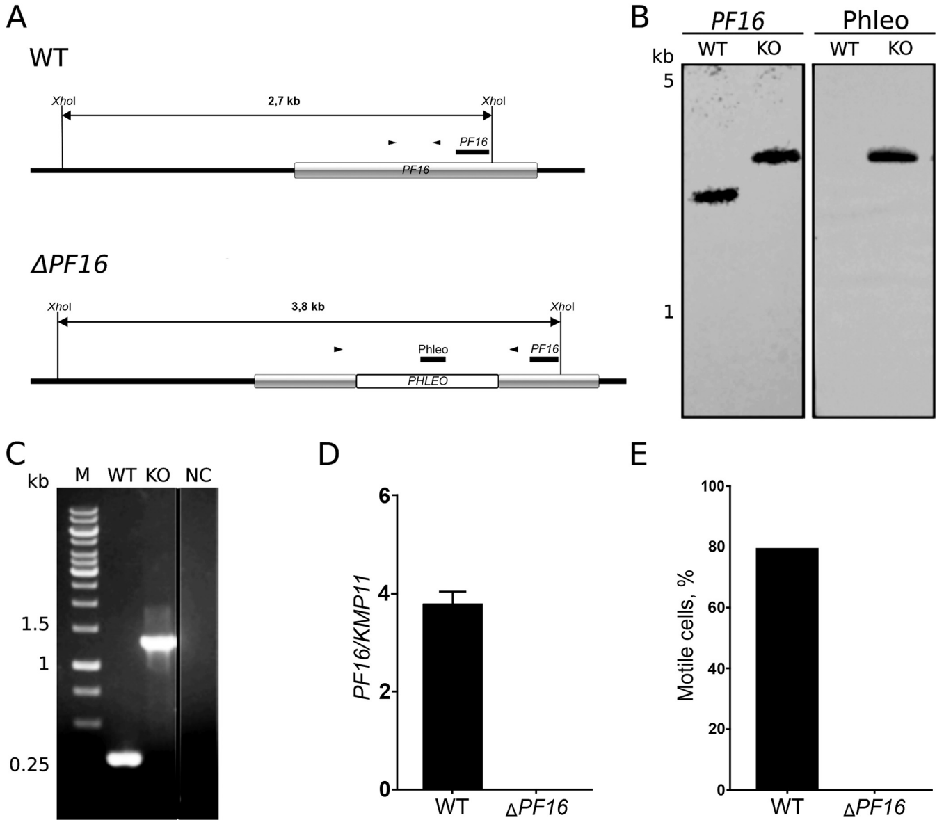
FIG 4 Genetic ablation of PF16 using CRISPR-Cas9-mediated approach in N. esmeraldas . (A) Schematic representation of the wild-type (top) and recombined (bottom) PF16 alleles of N. esmeraldas . Expected sizes of DNA fragments after XhoI digestion and positions of the annealed probes and primers for diagnostic PCR are indicated. (B) Southern blot analysis of the XhoI -digested N. esmeraldas genomic DNA of the WT and PF16 -ablated strains with PF16 and Phleo probes. (C) Diagnostic PCR for the wild-type and recombined (KO) PF16 alleles of N. esmeraldas . NC, negative control. (D) RT-qPCR control for the wild-type and \Delta PF16 alleles of N. esmeraldas . (E) Percent motile cells in the wild type and \Delta PF16 N. esmeraldas .
